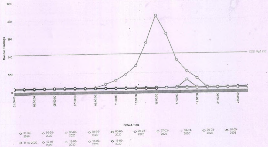
24 hrs Average data of COD Mg/l 250
